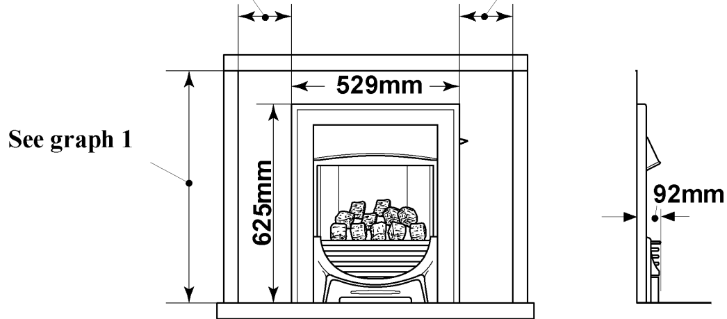
Figure 5. Appliance dimensions
